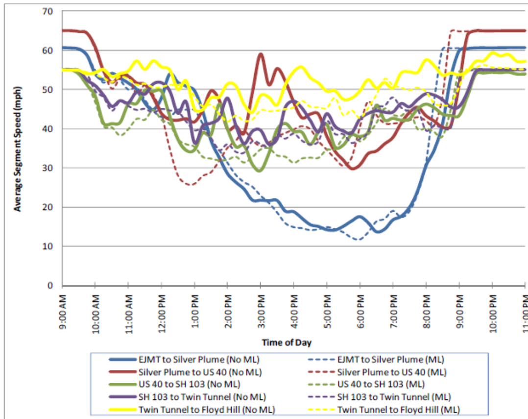
Figure 16. Eastbound Peak Period Speeds for 2015 Left Side PPSL
